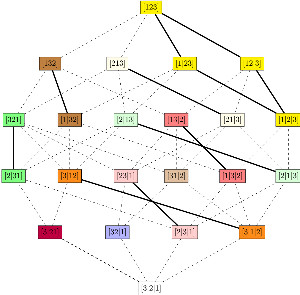
FIGURE 4. Cell decomposition and the Bruhat order for \mathcal{X}_3 .
